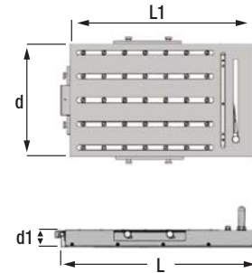
Die Changing Table (1Ton) Code: 1024-500670
