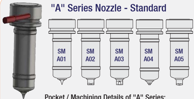
Pocket / Machining Details of "A" Series;
