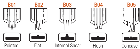
Nozzle Tip Types (BOX) & Gate Marks of Nozzle on the Product Surface;
