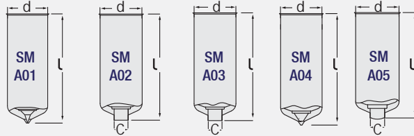
Nozzle Tip Types (AOX) & Gate Marks of Nozzle on the Product Surface;
