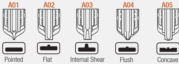
Nozzle Tip Types (AOX) & Gate Marks of Nozzle on the Product Surface;
