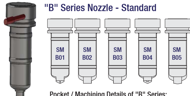
Pocket / Machining Details of "B" Series;
