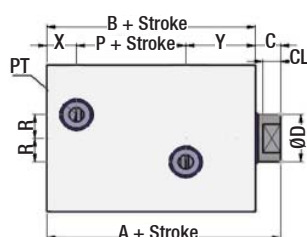
"THCF" Series Ø 32 - Ø 63
