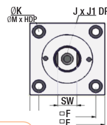
"THCFE" Series Ø 32 - Ø 63
