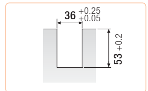
Machining Method for Plate
