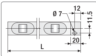
Outer Dimensions DL36 & DB36
