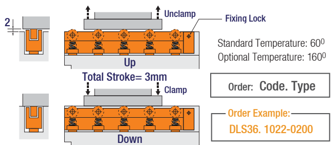
Code: DLS36 (with rollers)
