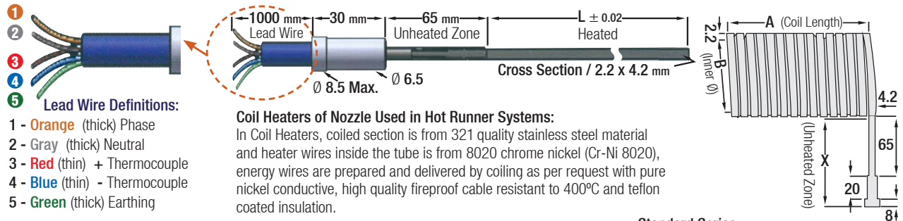
Coil Heater
